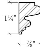
FEDERAL PANEL MOLD
