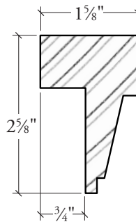
WAINSCOT CAP (WOWC006)
