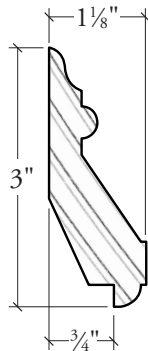
WAINSCOT CAP (WOWC002)
