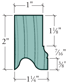
BRICK MOLD W/ KEY
