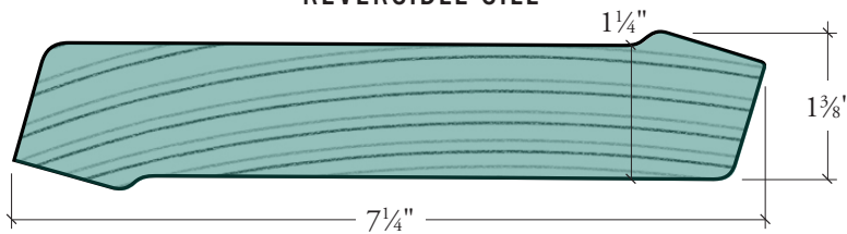
REVERSIBLE SILL
