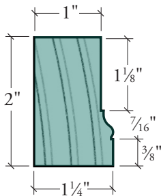
BRICK MOLD
