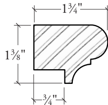
WAINSCOT CAP (WOWC003)
