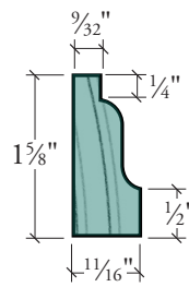
SHINGLE MOLD
